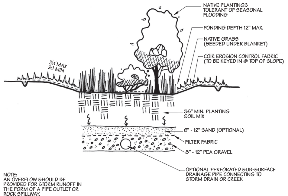
Bioretention basin
