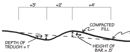
Water bar
