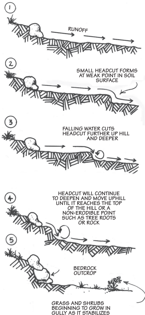
Headcut movement
