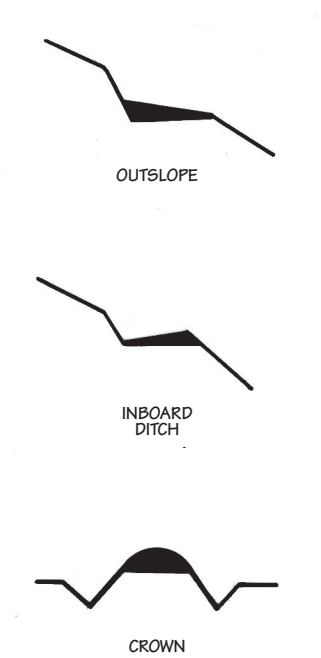
Types of surface road erosion
