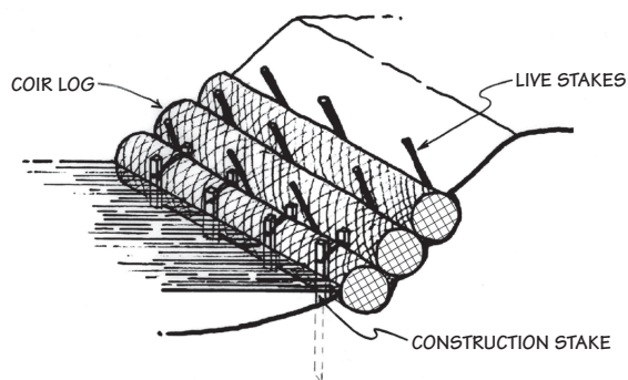
Coir log revetment with live willow staking
