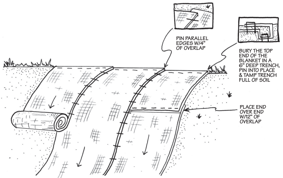
Erosion control fabric installation
