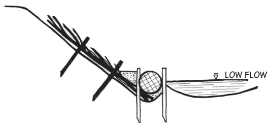
BRUSH MATTRESS WITH COIR LOG TOE
