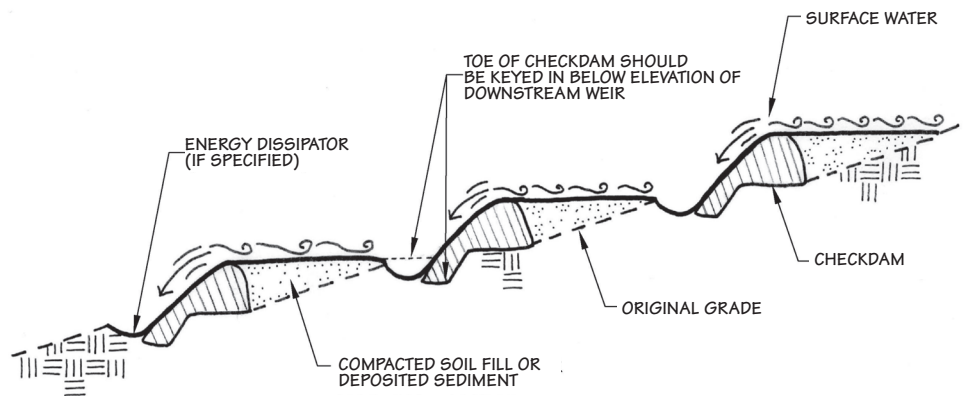
Checkdam placement
