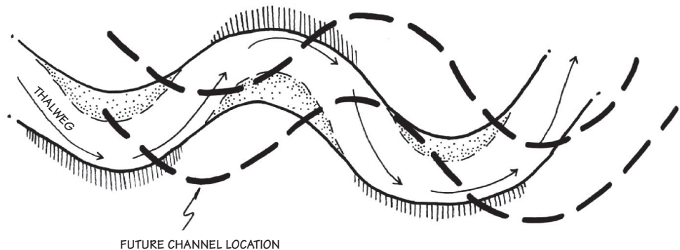
Channel migration
