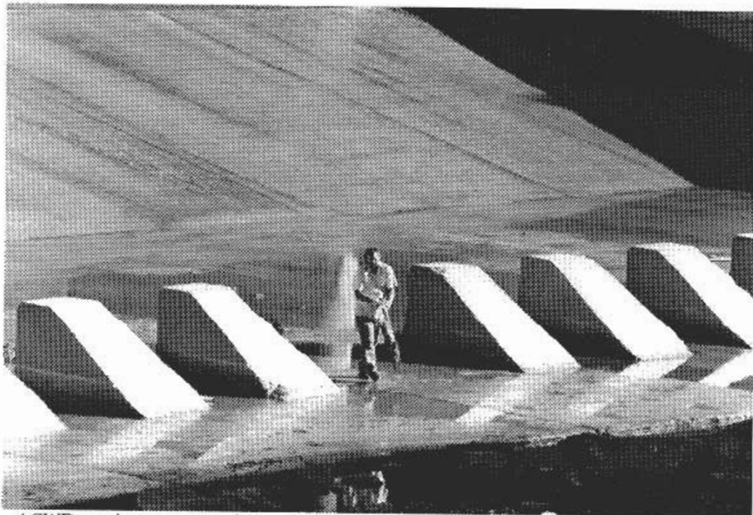
ACWD employee removes king salmon from channel. ACFCF weir is behind him. ACWD diversion fabric dam #1 is directly upstream of the weir. 11/28/97.
